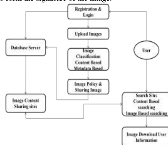
FIG: SYSTEM ARCHITECHTURE
