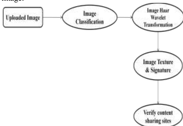
Fig: A3p- Content Based Classification
